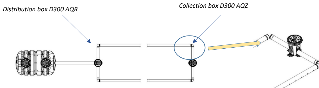
Figure 1: Collection box D300 AQZ – location in the drainage bed
